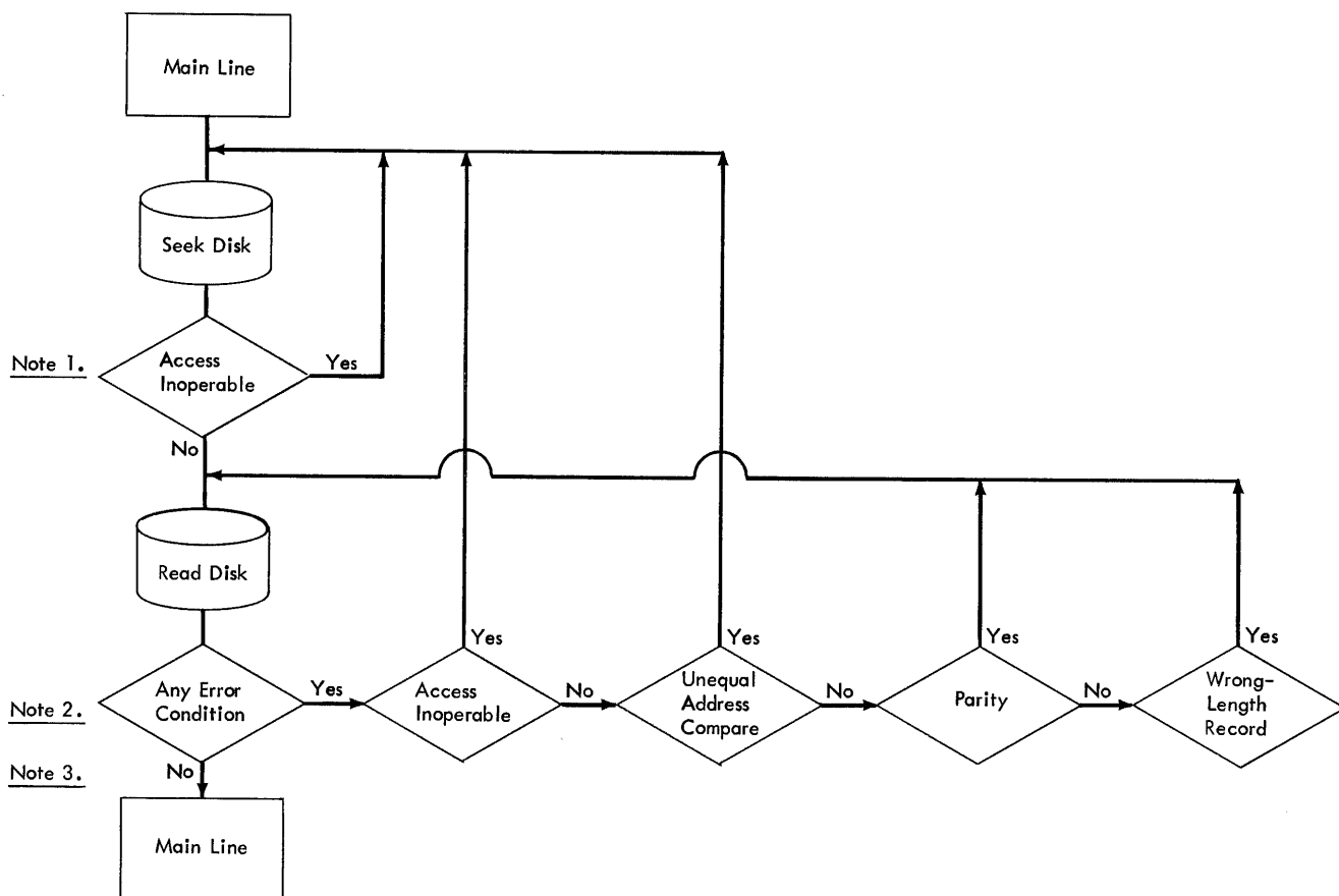
Figure G-13. IBM 1405 Disk Read Error Routine
