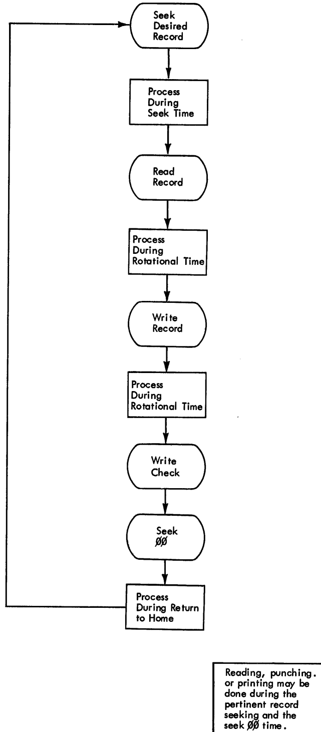
Figure G-34. Block Diagram for Dummy Seek Technique
