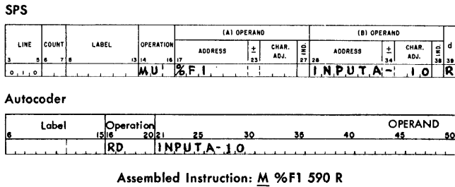
Figure G-20. Read Disk Sector
