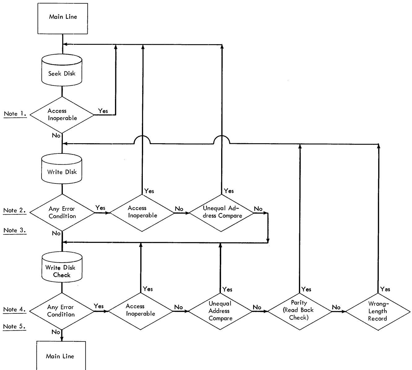
Figure G-14. IBM 1405 Disk Write Error Routine
