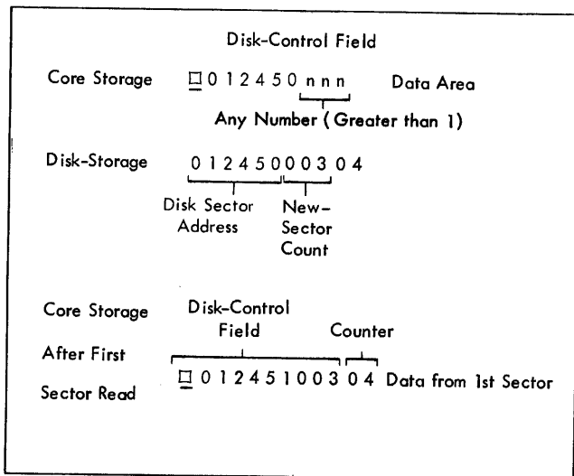
Figure G-42. Read Disk - Sector-Count Overlay Operation
