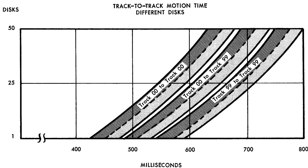
Figure G-10. Track-to-Track Motion Time Different Disks
