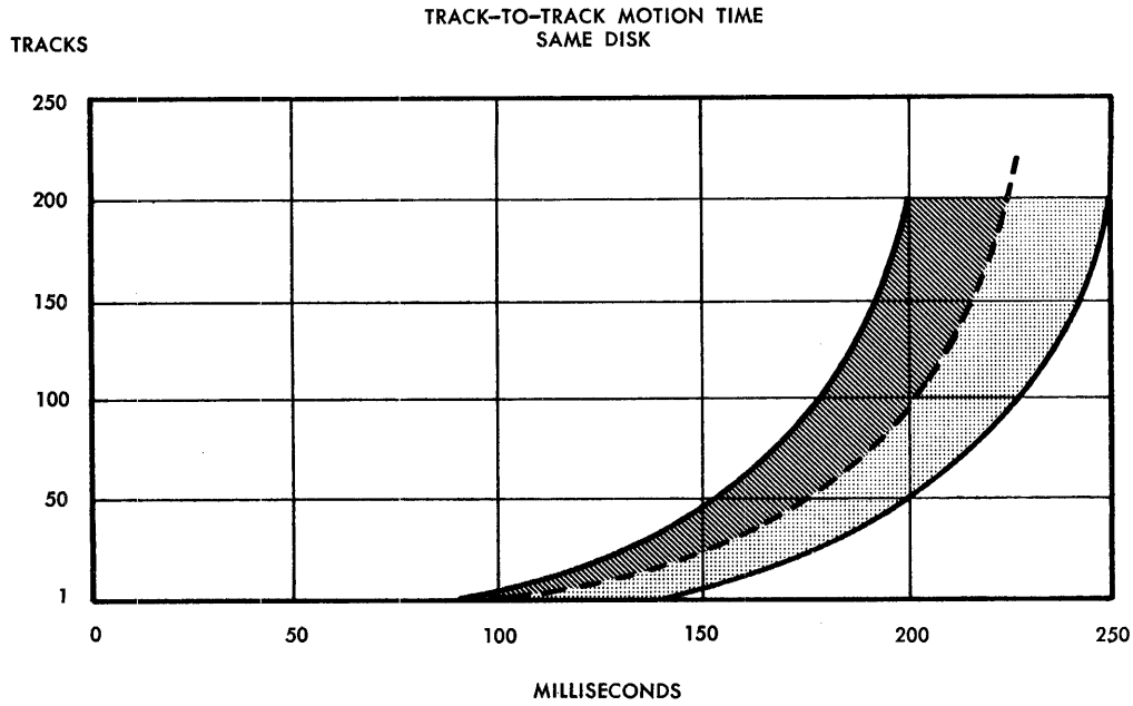
Figure G-11. Track-to-Track Motion Time Same Disks
