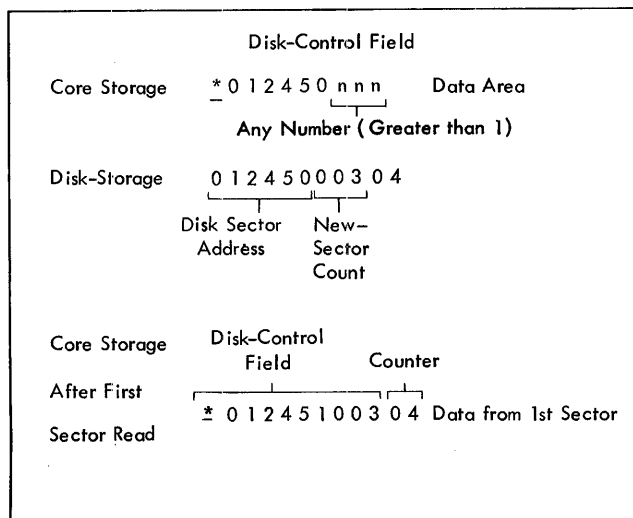
Figure G-22. Read Disks - Sector-Count Overlay Operation
