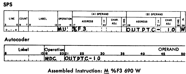
Figure G-28. Write Disk Check
