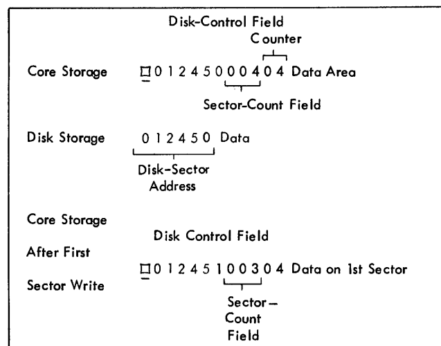
Figure G-46. Write Disk - Sector Count Overlay Operation
