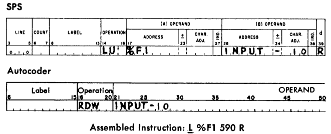
Figure G-21. Read Disk Sector with Word Marks
