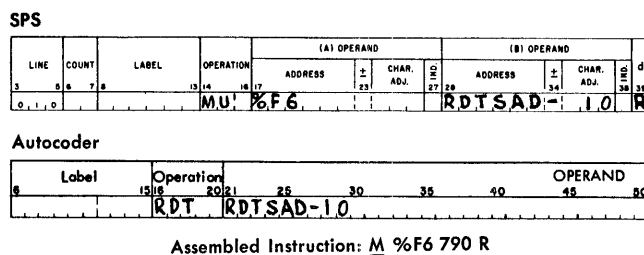
Figure G-29. Read Disk Track Sectors with Addresses
