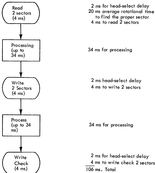
Figure G-35. Disk-Storage Timing for a 2-Sector Record
