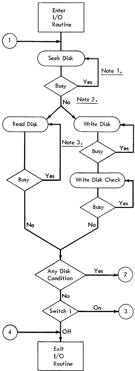
Figure G-36. IBM 1311 Operation and Error Routine
