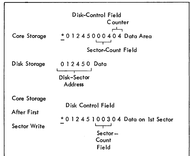
Figure G-26. Write Disk - Sector-Count Overlay Operations
