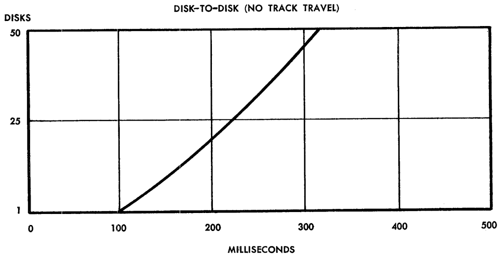
Figure G-12. Disk-to-Disk Travel (No Track Travel)
